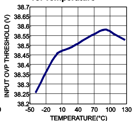
Input OVP Threshold vs. Temperature
