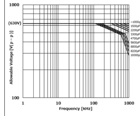
Chip(L×W): 3.2×1.6mm C0G(5C) Char. Rated Voltage:DC630V
