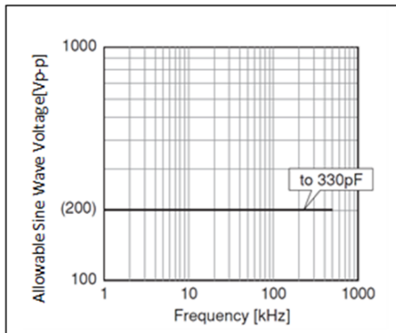
Chip(L×W): 2.0×1.25mm C0G(5C) Char. Rated Voltage:DC200V
