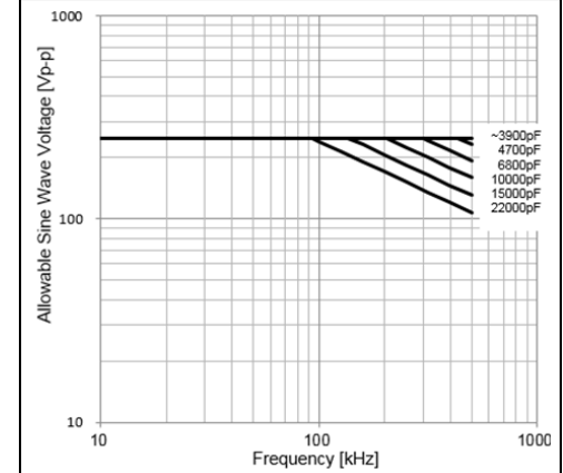
Chip(L×W): 3.2×1.6mm C0G(5C) Char. Rated Voltage:DC250V
