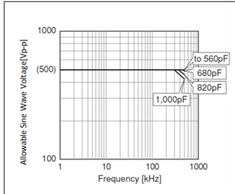
Chip(L×W): 3.2×1.6mm C0G(5C) Char. Rated Voltage:DC500V
