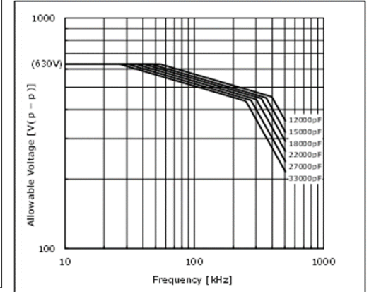
Chip(L×W): 3.2×2.5mm C0G(5C) Char. Rated Voltage:DC630V
