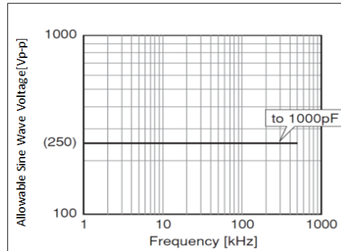
Chip(L×W): 1.6×0.8mm C0G(5C) Char. Rated Voltage:DC250V
