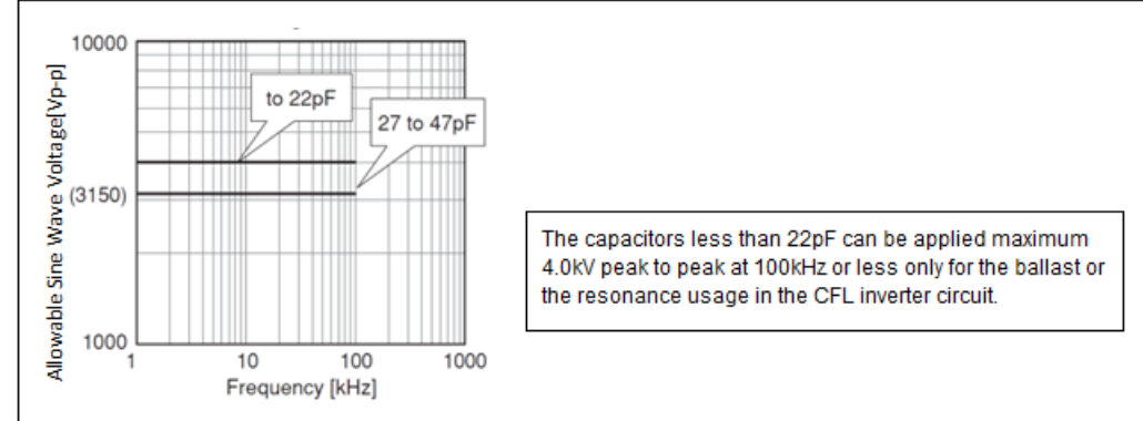
Chip(L×W): 4.5×2.0mm C0G(5C) Char. Rated Voltage:DC3.15kV
