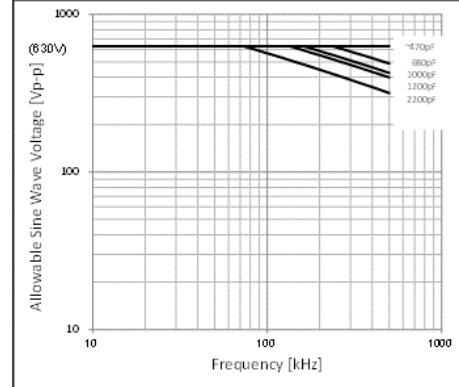
Chip(L×W): 2.0×1.25mm C0G(5C) Char. Rated Voltage:DC630V
