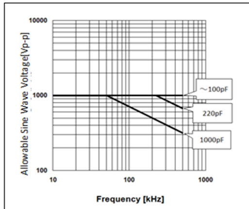
Chip(L×W): 3.2×1.6mm C0G(5C) Char. Rated Voltage:DC1kV
