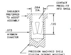
#34 CONTACT FOR .032"-.046" DIAMETER PINS ( \delta = .010 ) 4-FINGER, GROUP E (See page 248)
