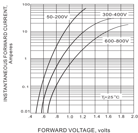
Fig.3 FORWARD CHARACTERISTICS
