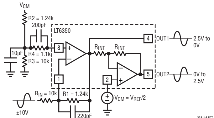
Figure 7. LT6350 Converting a \pm 10\text{V} Single-Ended Signal to a \pm 2.5\text{V} Differential Input Signal
