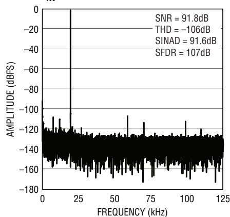
32k Point FFT f_S = 250\text{kpsps} , f_{IN} = 20\text{kHz}
