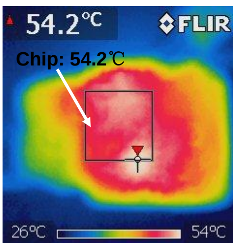
With dimmer at 50% dimming on phase
