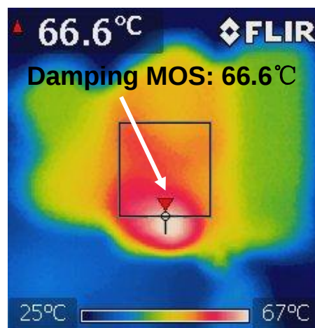
With dimmer at 50% dimming on phase
