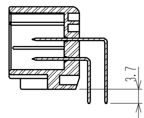
POWER CONTACT DIP DIMENSION
