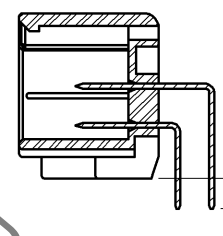
SIGNAL CONTACT DIP DIMENSION
