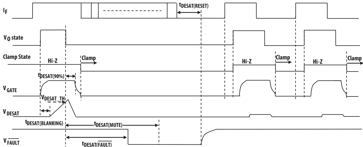
Figure 6. Circuit Behaviors During Overcurrent Event
