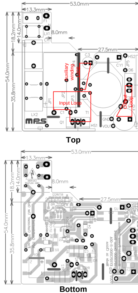
Figure 16: Recommended Layout
