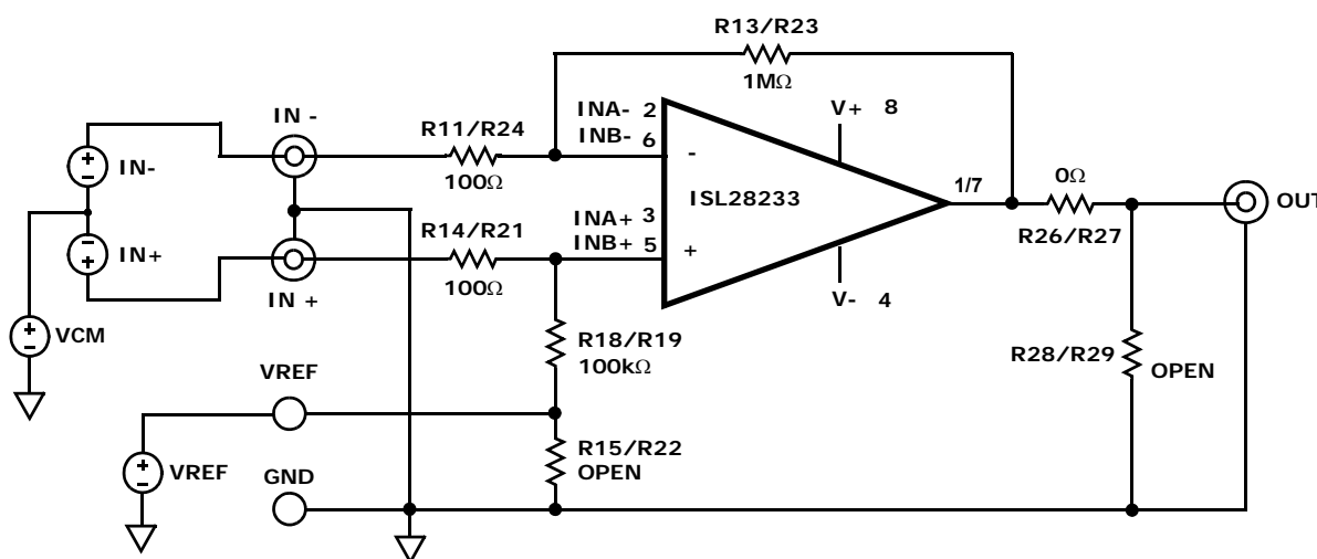
FIGURE 1. BASIC DIFFERENTIAL AMPLIFIER CONFIGURATION
