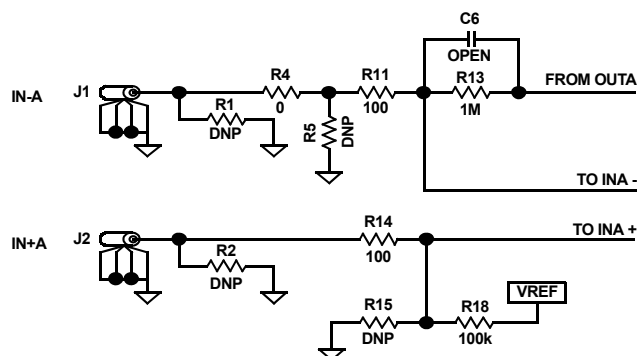
FIGURE 3. INPUT STAGE
