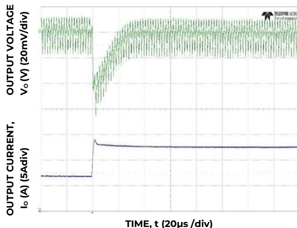
Figure 22. Transient Response to Dynamic Load Change from 50% to 100% at 12Vin, C_{out} = 4 \times 47\mu\text{F} + 1 \times 330\mu\text{F} CTune=1.2nF, RTune=300Ω
