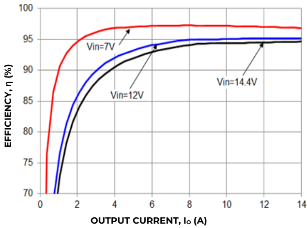
Figure 31. Converter Efficiency versus Output Current.
