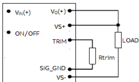
Figure 42. Circuit configuration for programming output voltage using an external resistor.
