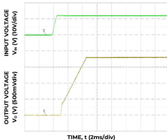
Figure 18. Typical Start-up Using Input Voltage ( V_{IN}=12V , I_o = I_{o,max} ).
