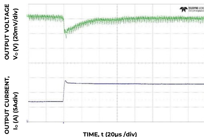
Figure 10. Transient Response to Dynamic Load Change from 50% to 100% at 12Vin, C_{out}=8 \times 47\mu\text{F}+3 \times 330\mu\text{F} CTune=3.9nF, RTune=300Ω
