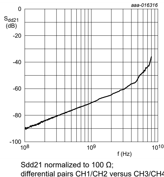
Fig. 3. Mixed-mode differential NEXT crosstalk; typical values
