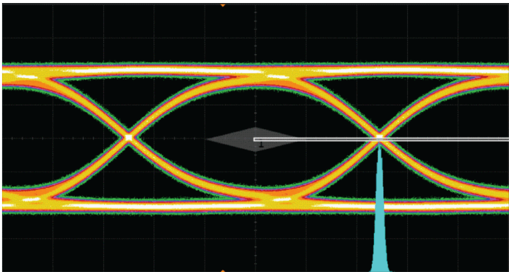
Fig. 5. HDMI 2.0 TP1 eye diagram, PCB with device
