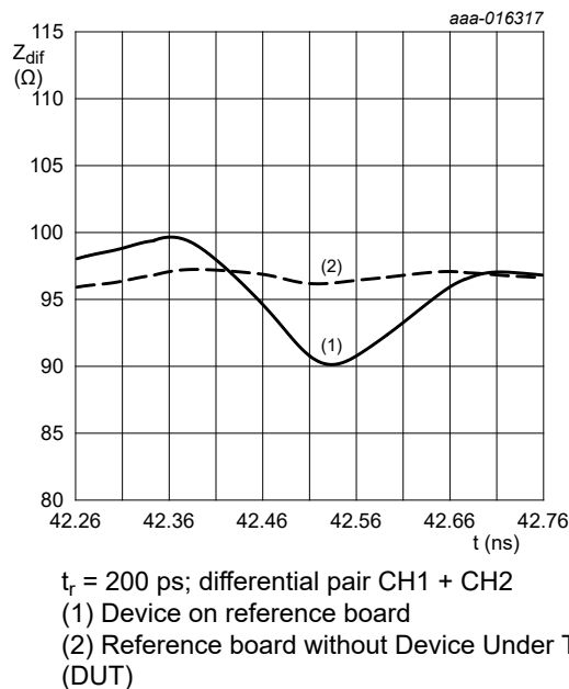
Fig. 4. Differential Time Domain Reflectometer (TDR) plot; typical values
