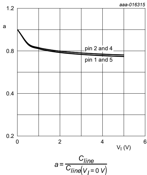
Fig. 2. Relative capacitance as a function of input voltage; typical values
