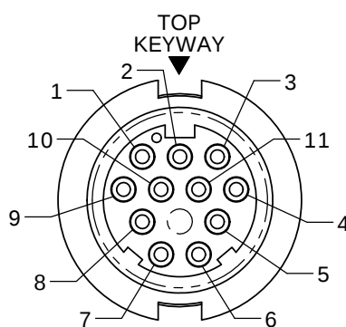
FACE VIEW W3282-11PG-5XX(W)
