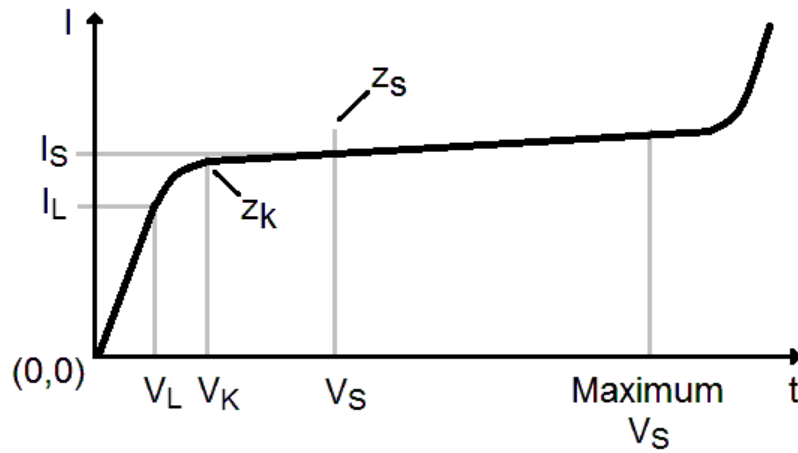
FIGURE 1 – CURRENT-REGULATOR CHARACTERISTICS
