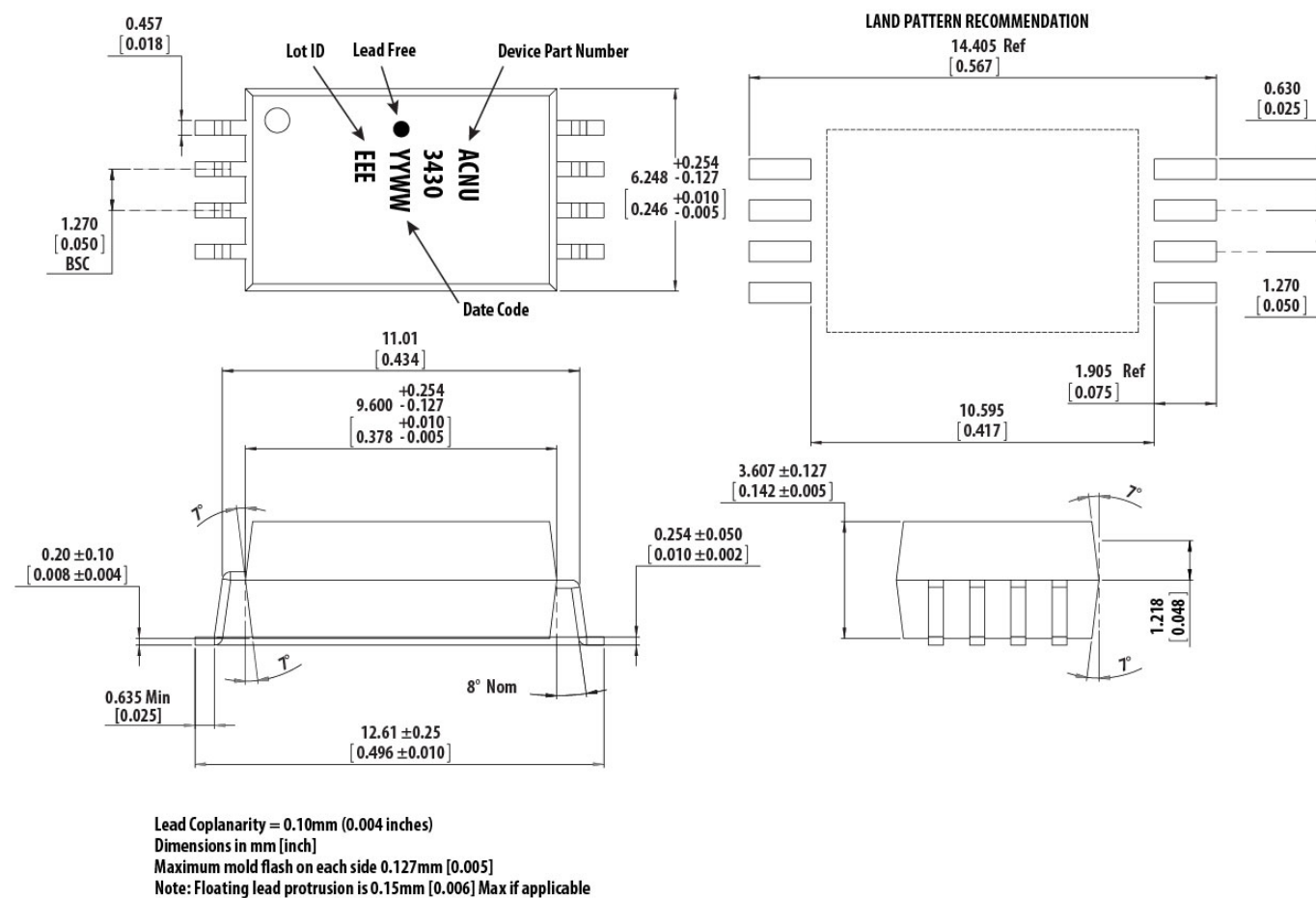
Figure 2: ACNU-3430 Outline Drawing (11-mm SSO8 Package)
