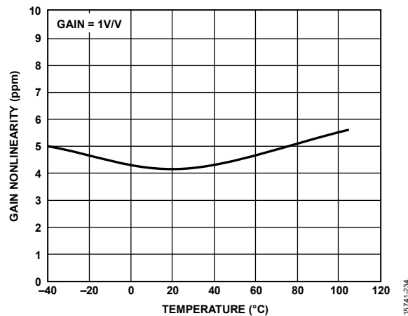
Figure 22. Gain Nonlinearity vs. Temperature
