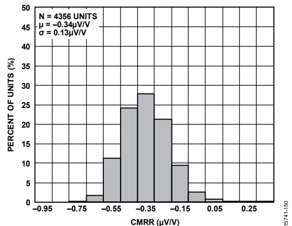
Figure 25. CMRR Distribution (Gain = 1 V/V)
