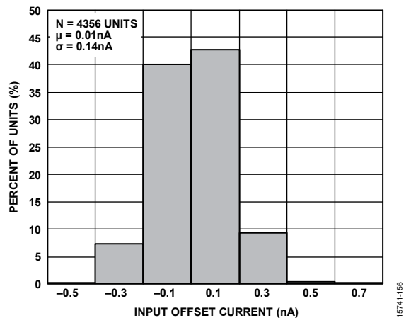
Figure 30. Input Offset Current Distribution
