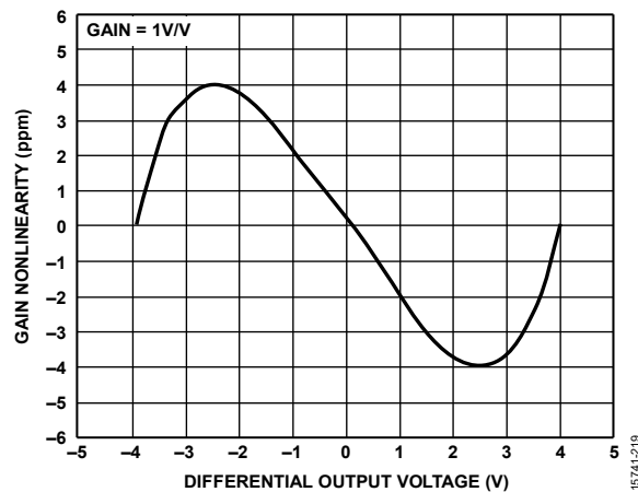
Figure 19. Gain Nonlinearity
