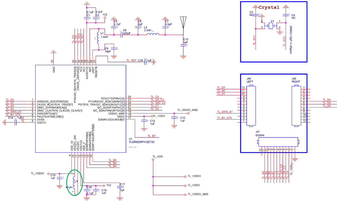
Figure 16- 2 Schematic
