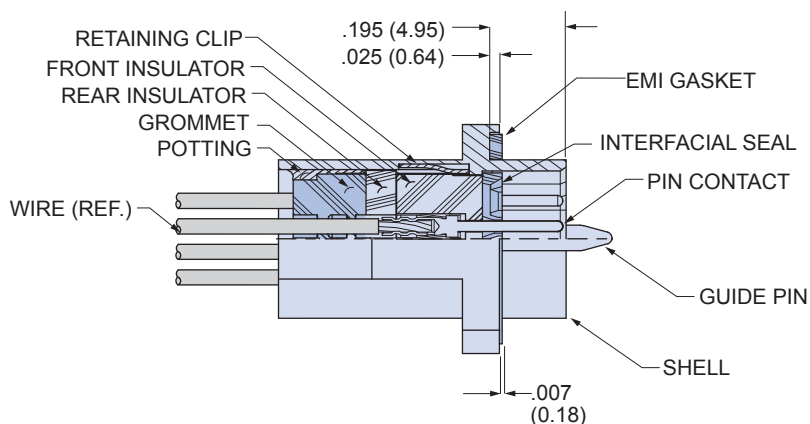
CROSS-SECTIONAL VIEW OF 790-026P
