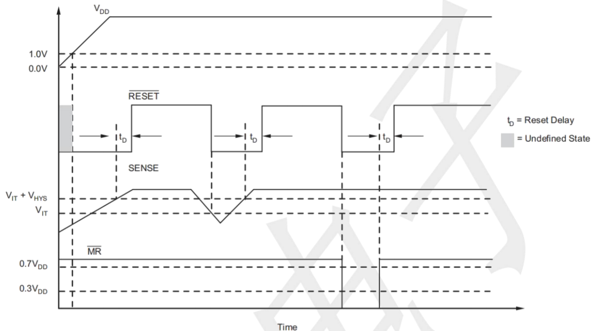
\overline{MR} and \overline{SENSE} Reset Timing Diagram
