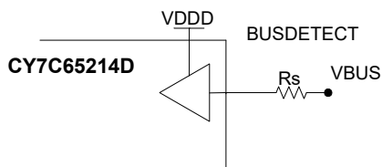
Figure 10. GPIO VBUS Detection, VBUS = VDD
