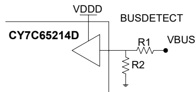
Figure 11. GPIO VBUS Detection, VBUS > VDD
