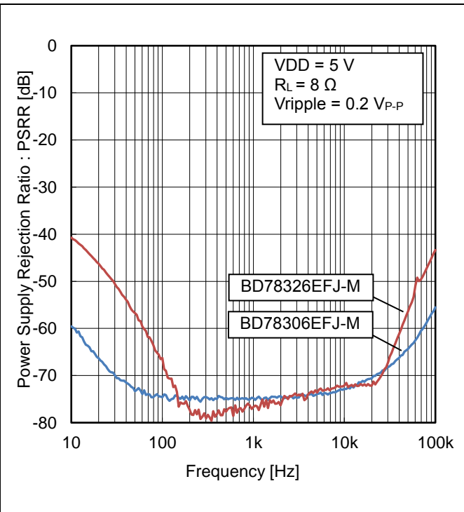
Figure 14. Power Supply Rejection Ratio vs Frequency
