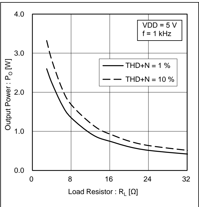
Figure 12. Output Power vs Load Resistor
