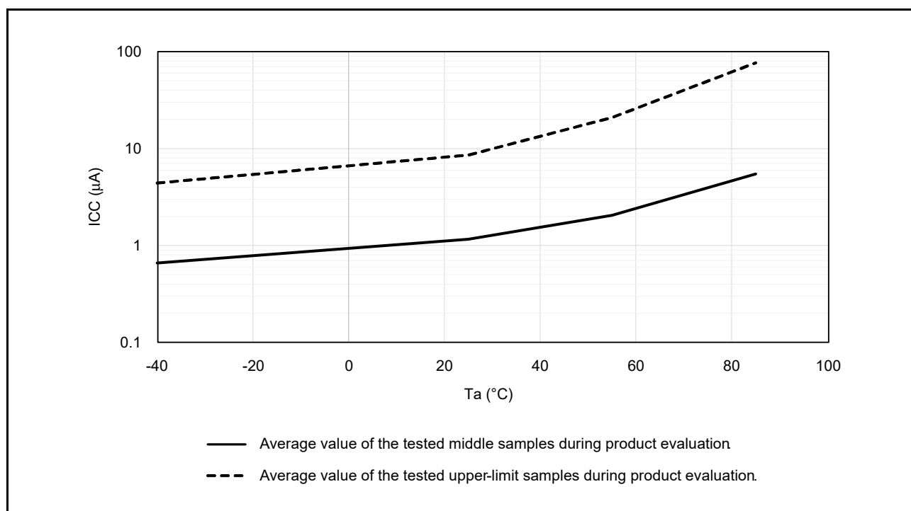
Figure 5.3 Temperature Dependency in Software Standby Mode (Chip Version A) (Reference Data)
