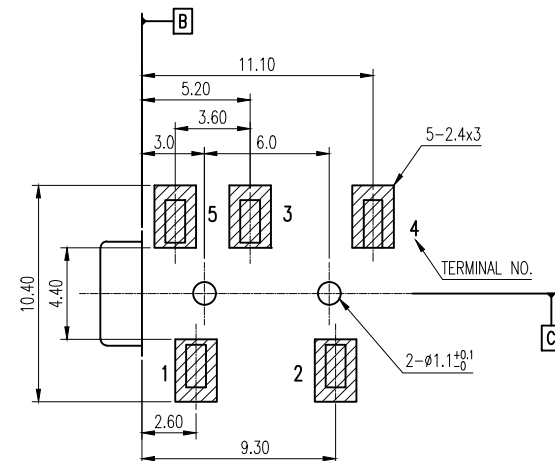
P.C.B Layout Dimension (Tolerance: \pm 0.1 ) (Recommend min. Dimension) (top view)
