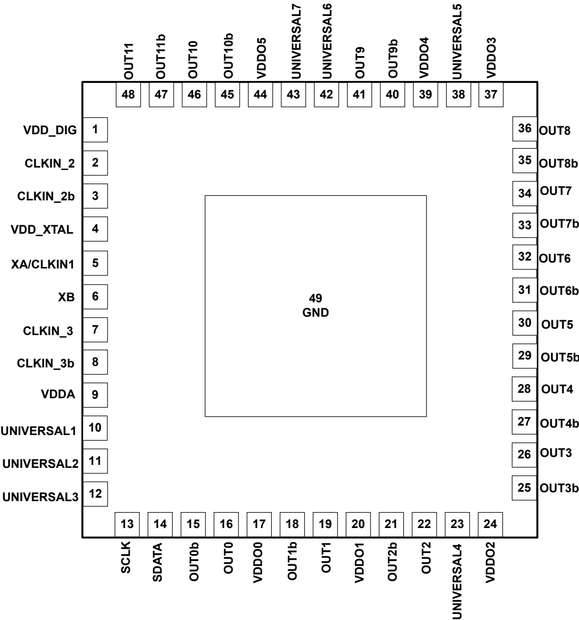
Figure 6.1. 48-QFN
