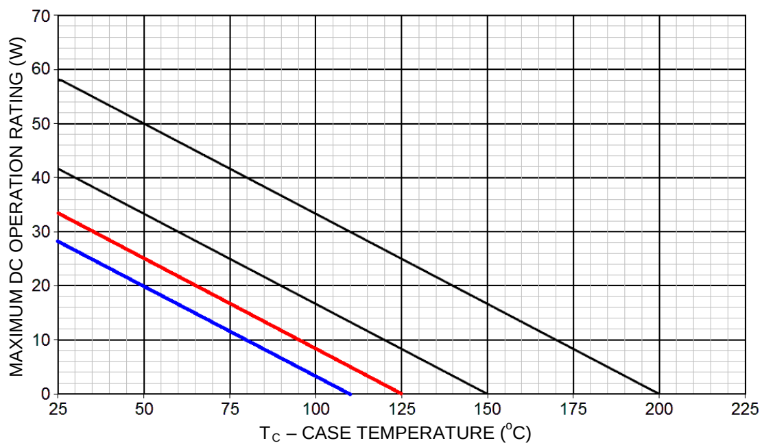
FIGURE 1 Temperature-Power Derating
