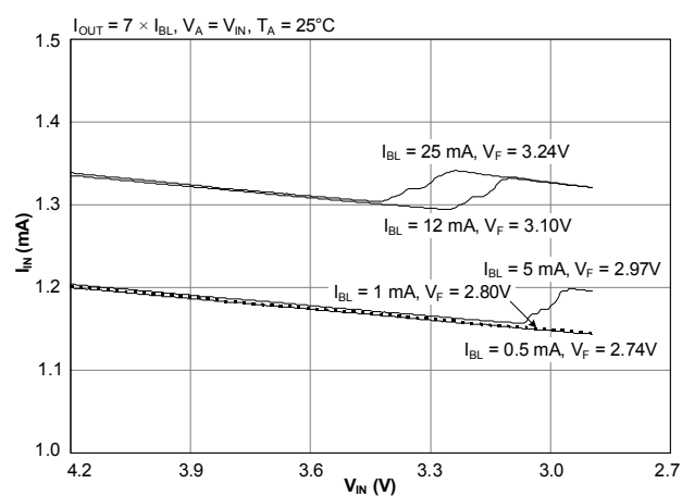
Supply Current (7 LEDs)
