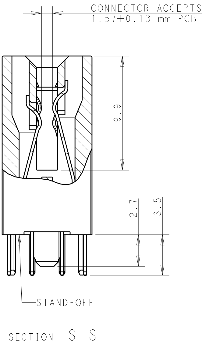
SECTION S-S
