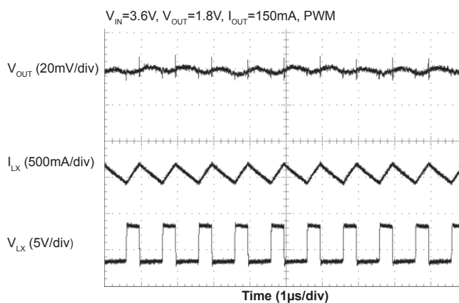
PWM Operation
