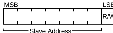
Figure 13: 7-Bit Address
