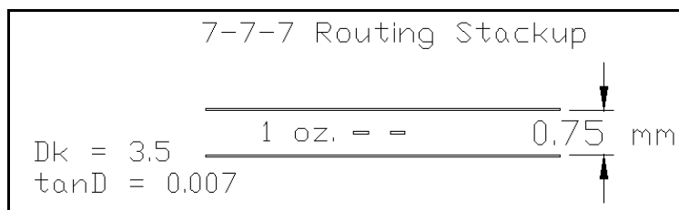
Figure 63: 7-7-7 Routing
