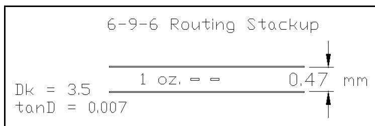
Figure 74: 6-9-6 Routing
