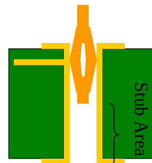
Figure 5: Via Stub
