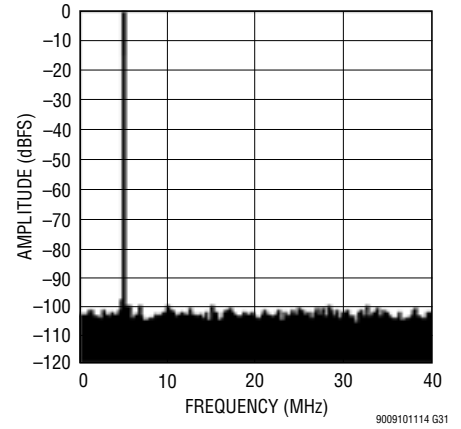
LTM9009-14: 8k Point FFT, f_{IN} = 5\text{MHz} , -1\text{dBFS} , 80Msps
