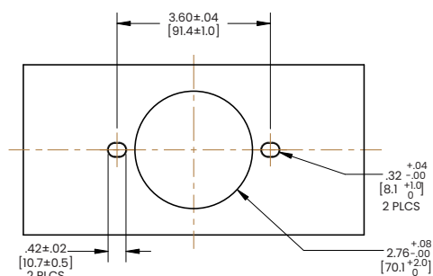
MOUNTING PANEL
