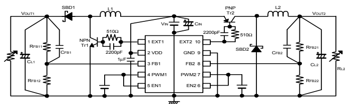
Circuit ①
