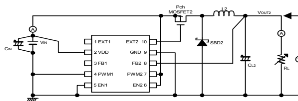
Circuit ⑦
