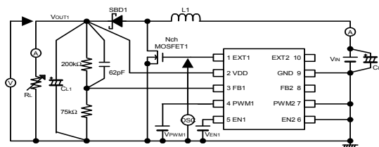
Circuit ⑤
