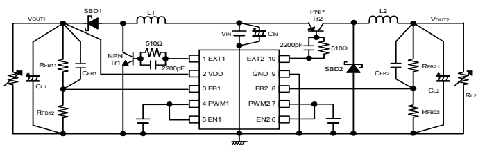
Circuit ②
