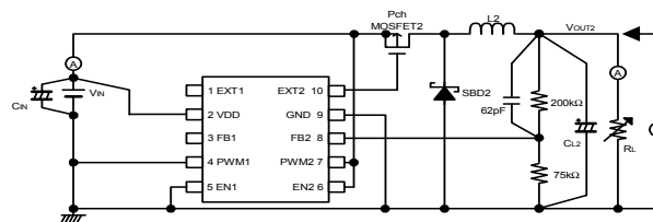
Circuit ⑧
