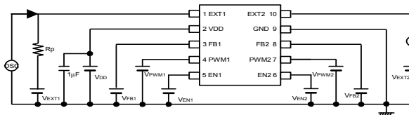
Circuit ⑦
