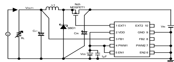
Circuit ④
