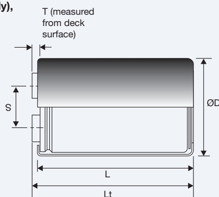
ALS30 Clamp Mounting
