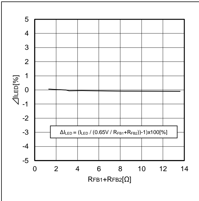
Figure 5. ΔILED vs RFB1+RFB2
