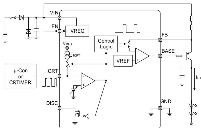
Figure 16. PWM Dimming Operation using external signal
