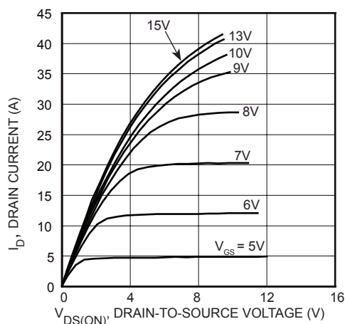
FIGURE 1, Output Characteristics
