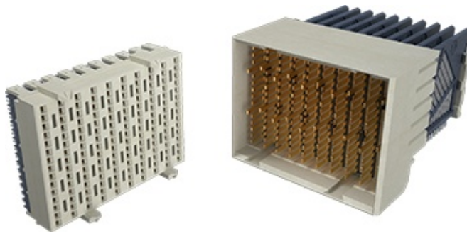
Vertical Receptacle
