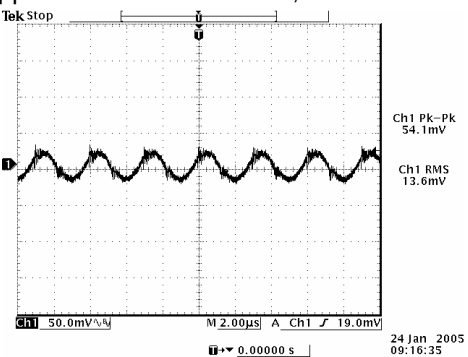
Ripple and noise at full load, 3.3 V/46 A output
