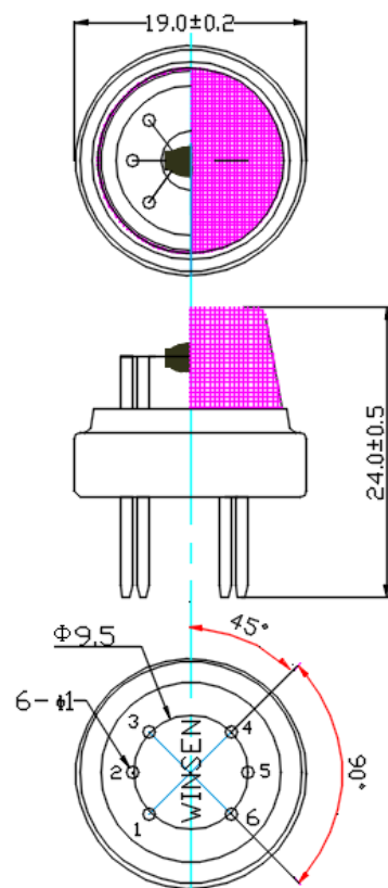
Fig1.Sensor Structure
