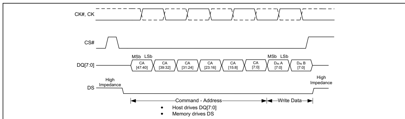
Figure 4 Write operation [4, 9, 10]
