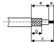
STRIPPING DIMENSIONS
