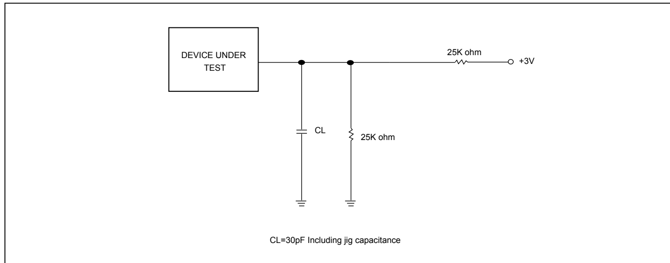
Figure 82. OUTPUT LOADING
