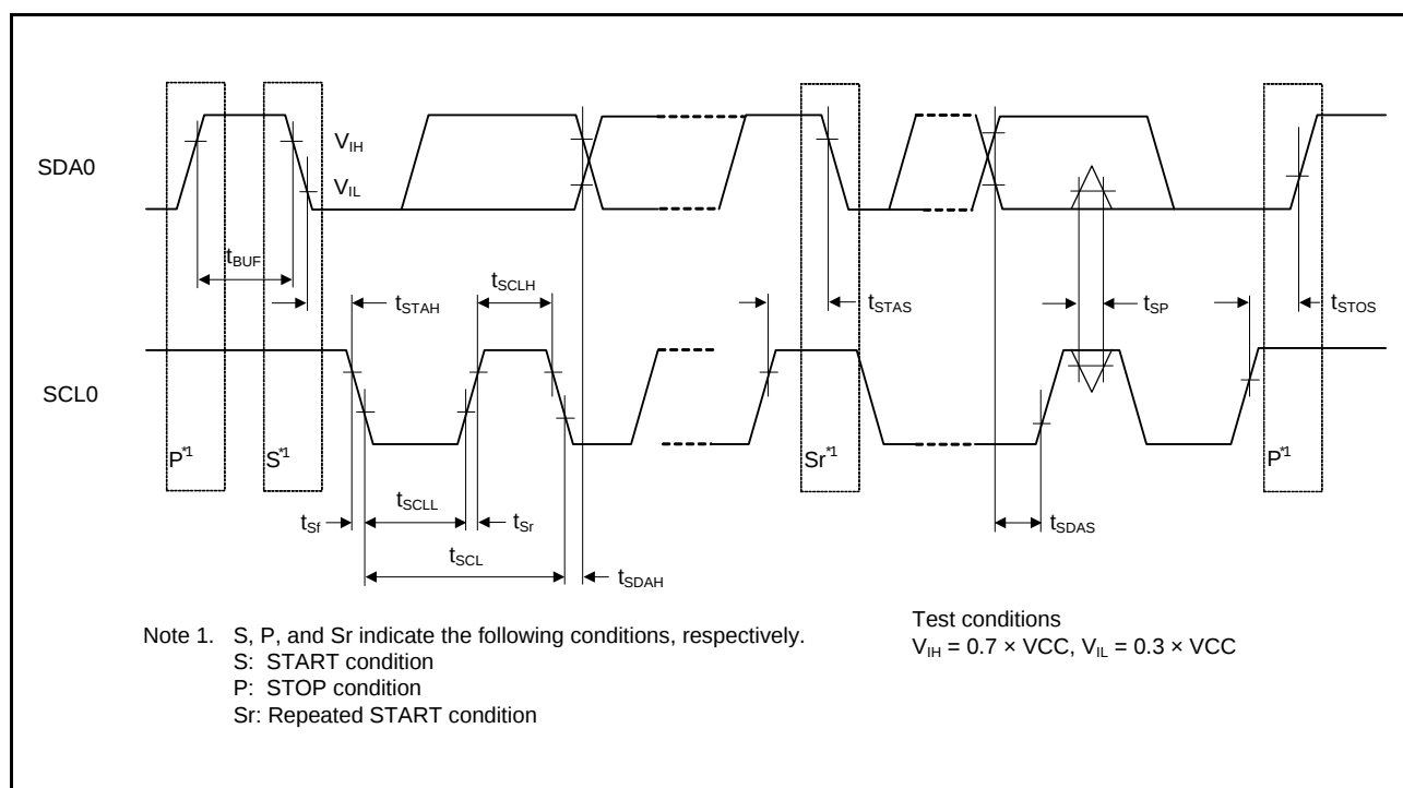
Figure 5.49 IIC Bus Interface Input/Output Timing and Simple I 2 C Bus Interface Input/Output Timing
