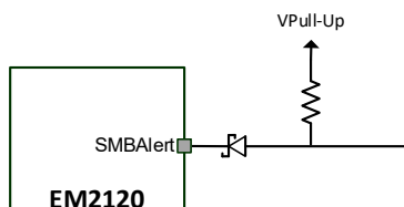
Figure 7: SMBAlert Pin Low Voltage Pull-up Option
