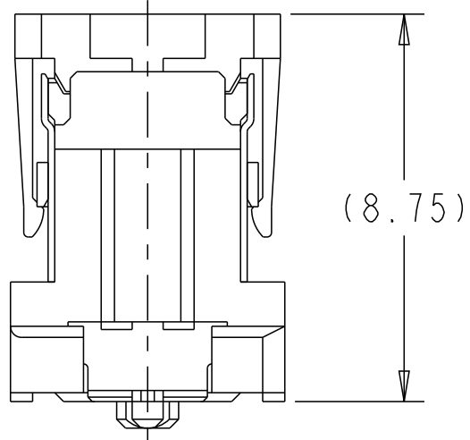
CONNECTOR DETAIL
