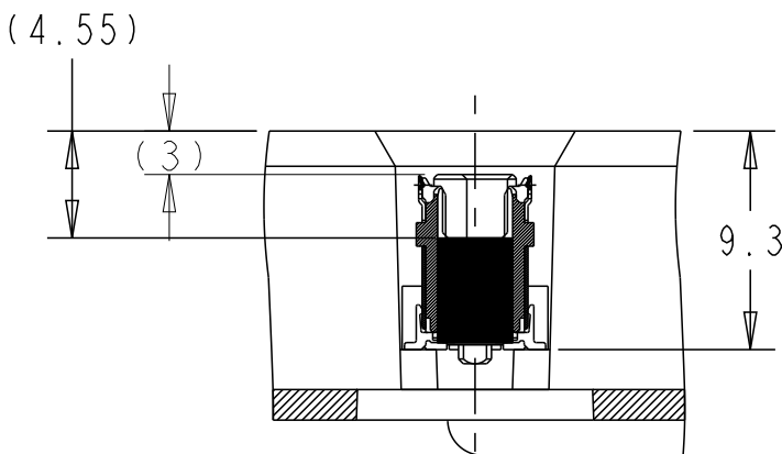
SECT. E-E (SCALE 2:1)
