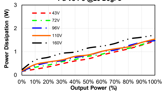
EC6AW-110D15 Pd Vs Po @25 Deg. C
