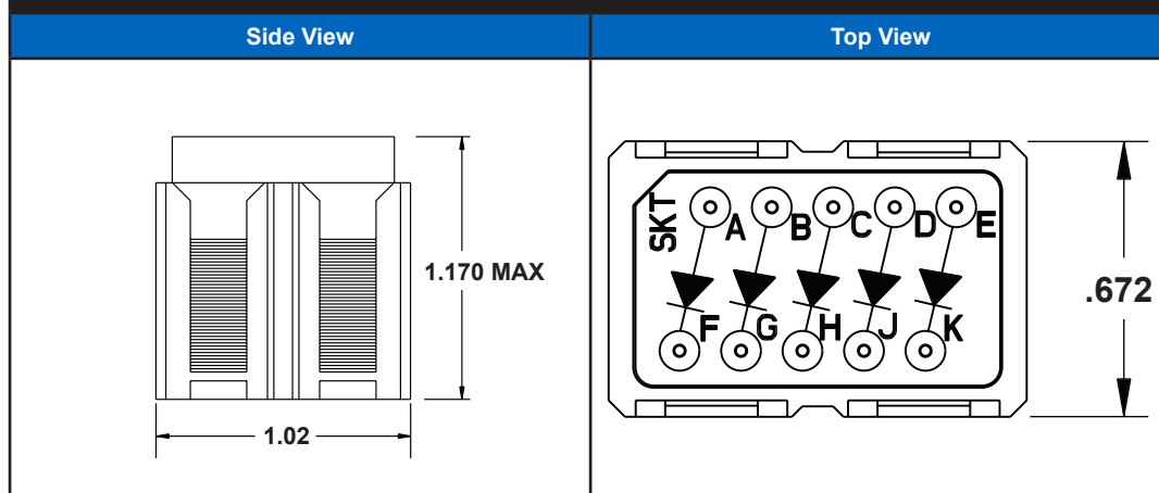
Socket Junction Module Dimensions
