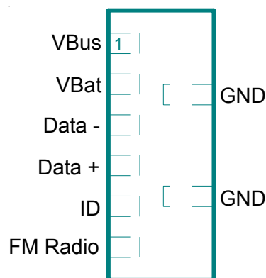
Figure 1- Pin Configuration
