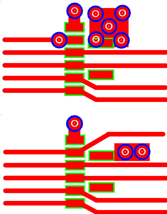
Figure 2 - Layout Examples
