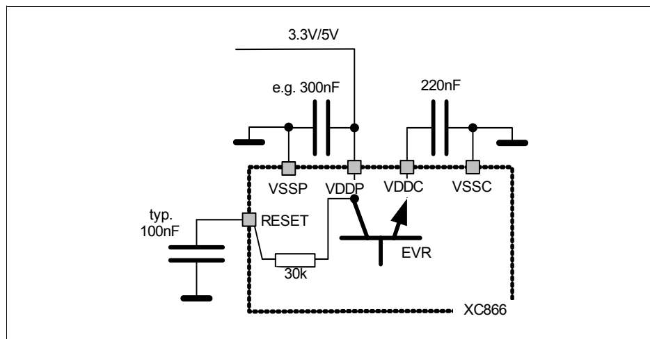
Figure 21 Reset Circuitry
