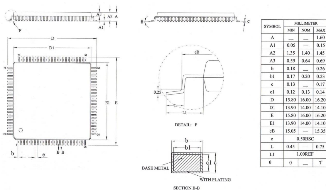
Figure 15 Mechanical Outline of 100LQFP
